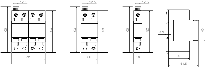
Dimensions:
