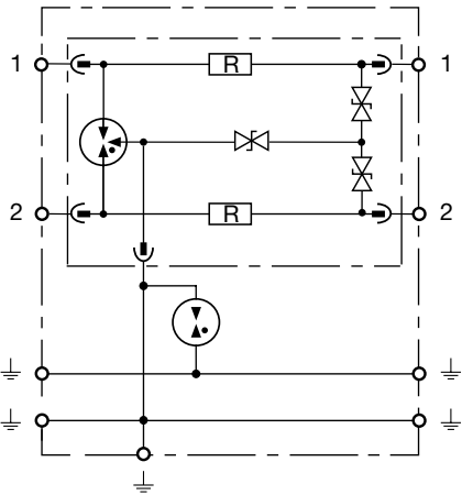
Circuit Diagram:
