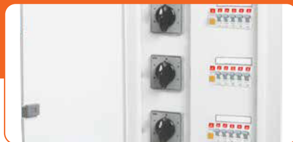
Manual phase selector DB which allows shifting to healthy phase using phase selector switches
