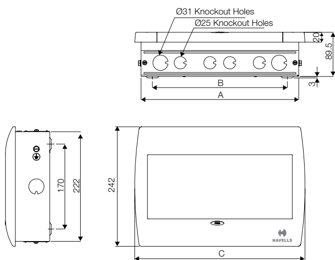
Dimensions SPN (in mm)
